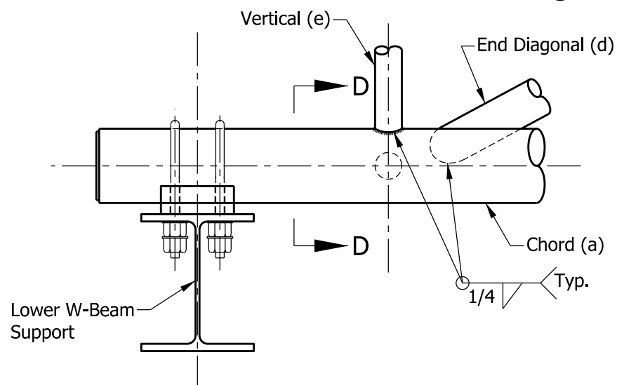
DETAIL A SUPPORT END DETAIL FOR EXTERIOR SECTION
