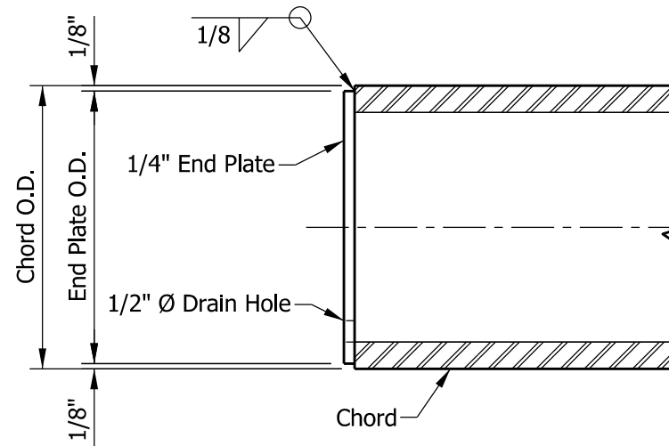
SECTION G-G
