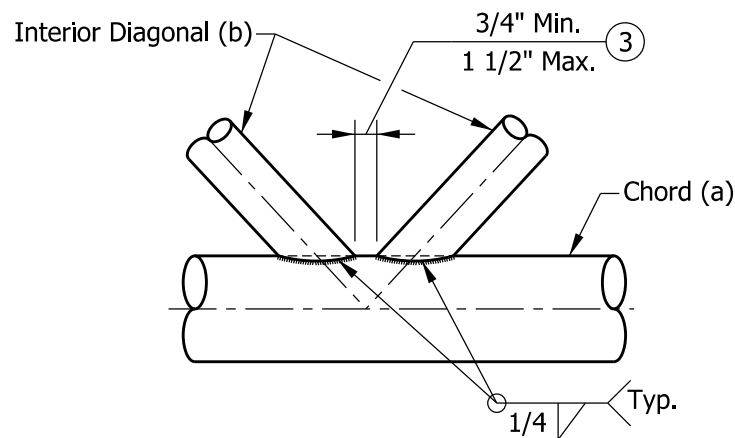
DETAIL B TYPICAL PANEL CONNECTION
